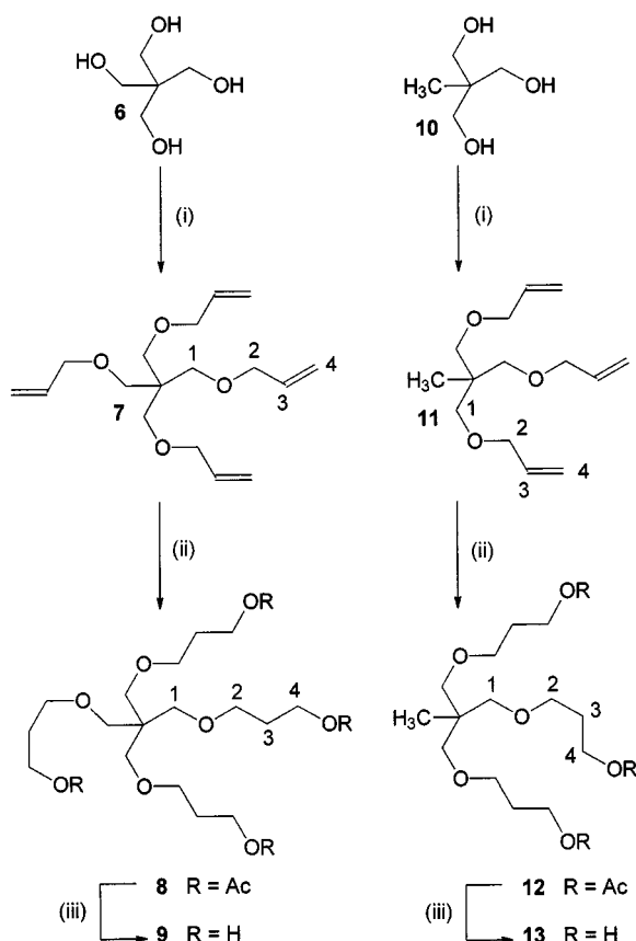
Scheme 3. (i) Allyl bromide, aq. NaOH, TBABr, 59% for 7 , 47% for 11 ; (ii) 9-BBN, THF, then NaOH and H 2 O 2 , then Ac 2 O, pyridine, 87% for 8 , 84% for 12 ; (iii) NaOMe, MeOH, quant.
