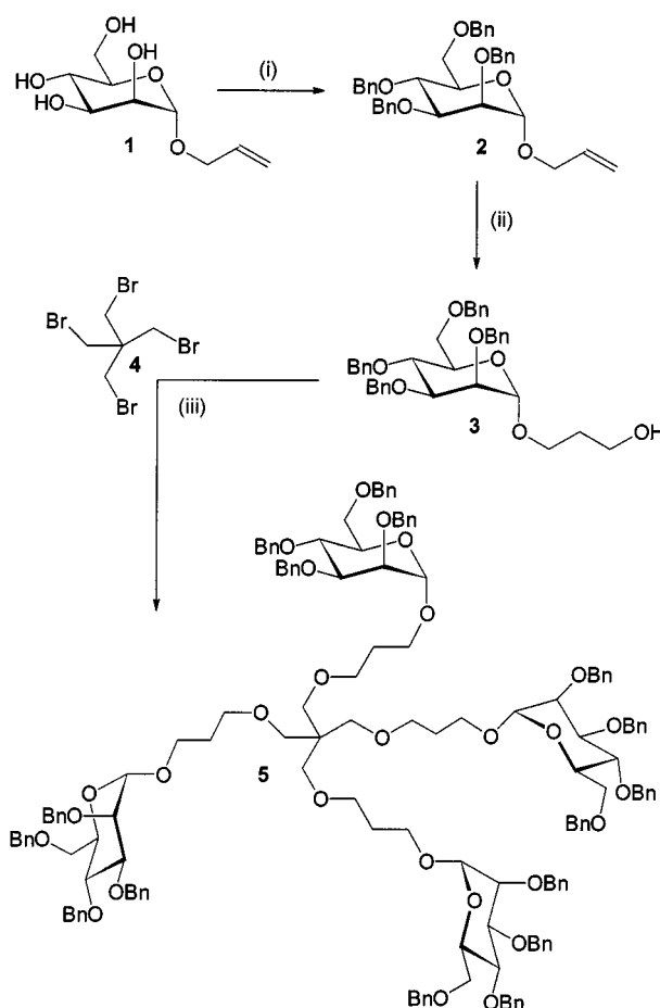
Scheme 2. (i) BnBr, NaH, DMF, 86%; (ii) 9-BBN, THF, then NaOH and H_2O_2 , 91%; (iii) NaH, diglyme, 62%
