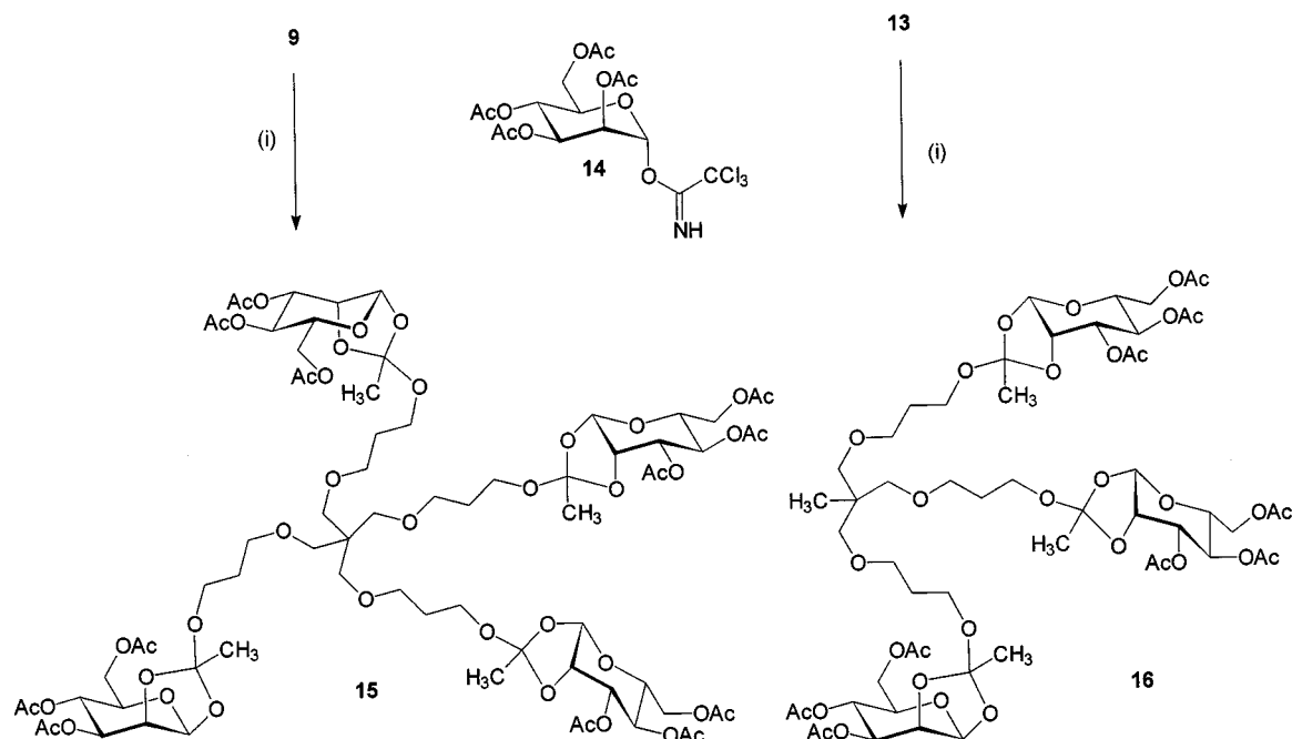
Scheme 4. (i) TMSOTf; for 15 in acetonitrile, 64%; for 16 in toluene, 54%
