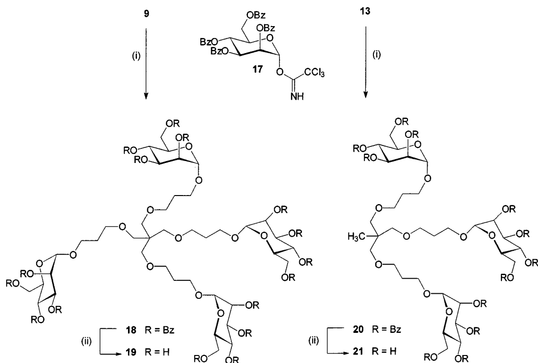
Scheme 5. (i) \text{CH}_2\text{Cl}_2 , TMSOTf, 92% for 18 , 95% for 20 ; (ii) NaOMe, MeOH, quant.
