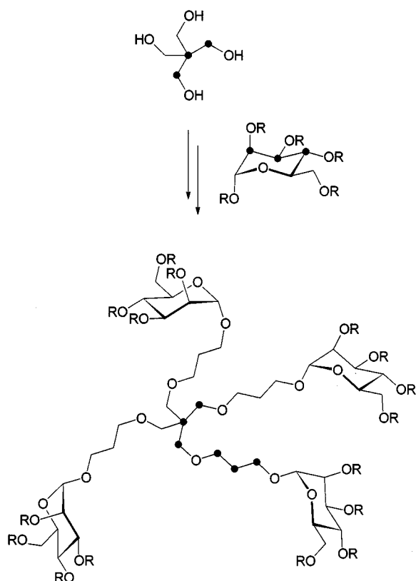
Scheme 1. Pentaerythritol-based cluster glycosides as depicted were designed to serve as high mannose-type glycan mimetics, in which C_3 spacers, highlighted by black dots, are thought to substitute monosaccharide units
